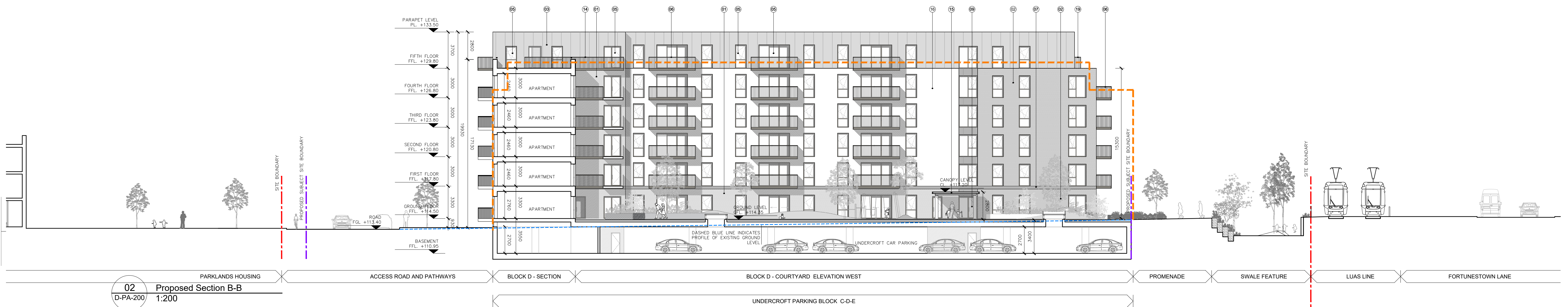
01 Proposed Section A-A D-PA-200 1:200
